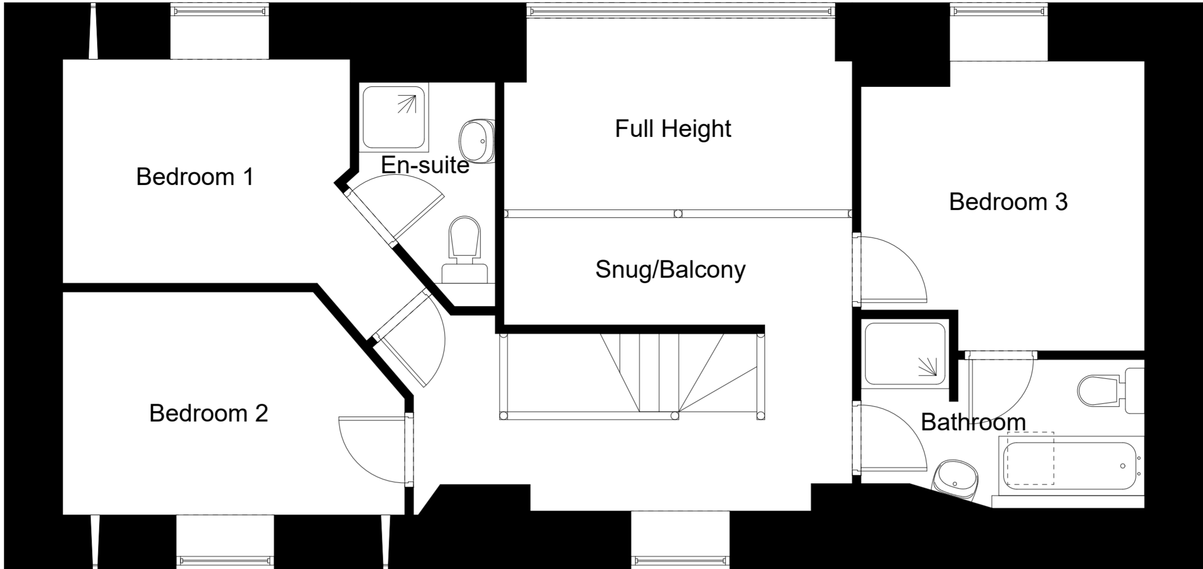
First Floor
