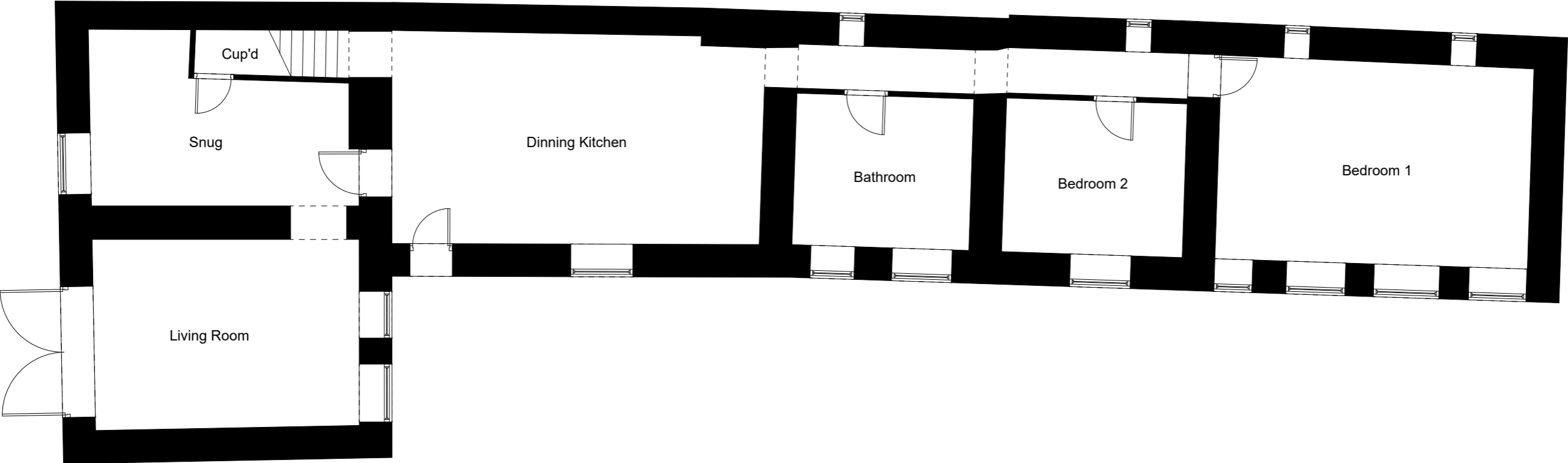
Ground Floor
